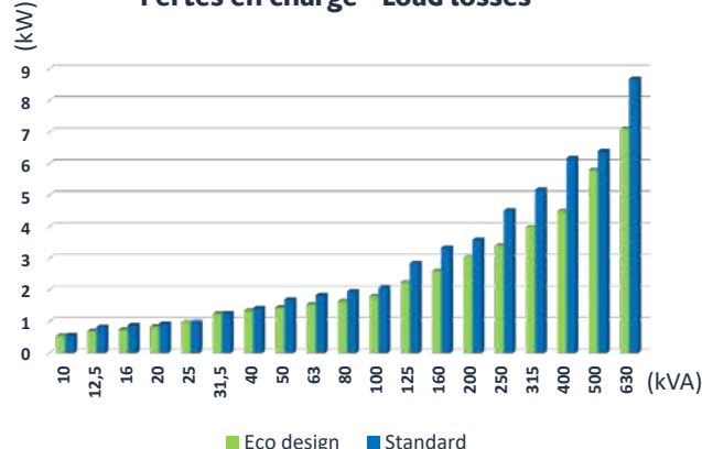
Pertes en charge - Load losses
